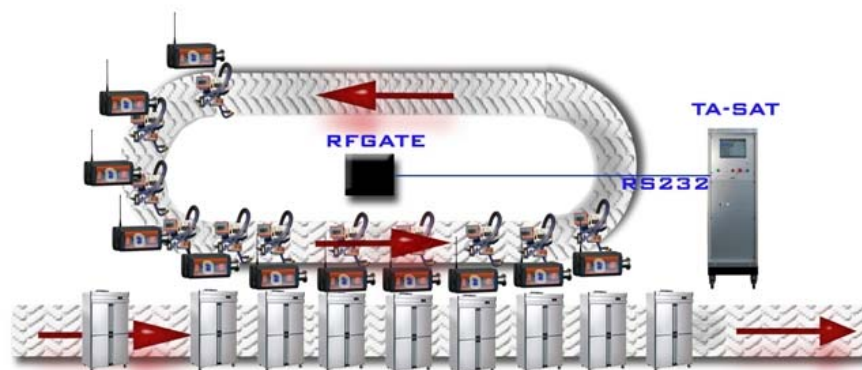
Vacuum Pump Carousel with TA100RF Heads, RF Gate and TA-SAT
